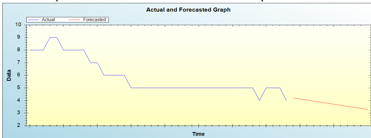
Figure 4: Out-of-sample forecast for X: actual and forecasted graph
