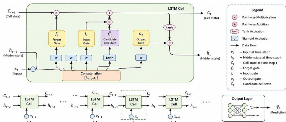
Figure 2. Structure of the LSTM forecasting model
