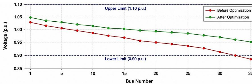
Figure 4. Power-loss reduction and voltage-profile improvement after optimization
