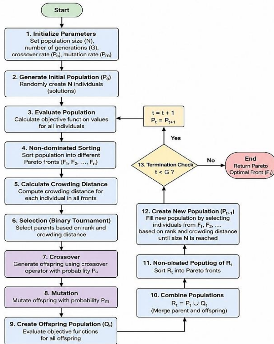
Figure 3. NSGA-II optimization procedure
